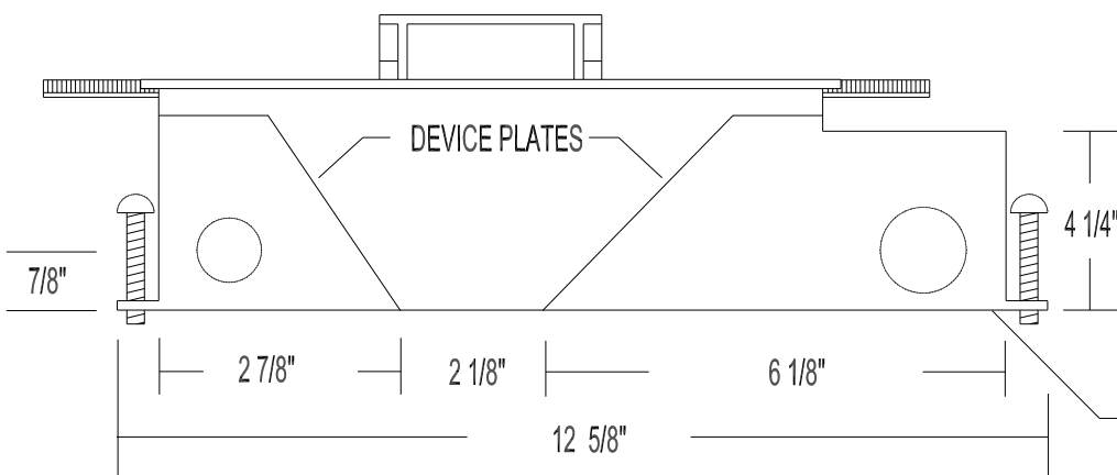
END VIEW
