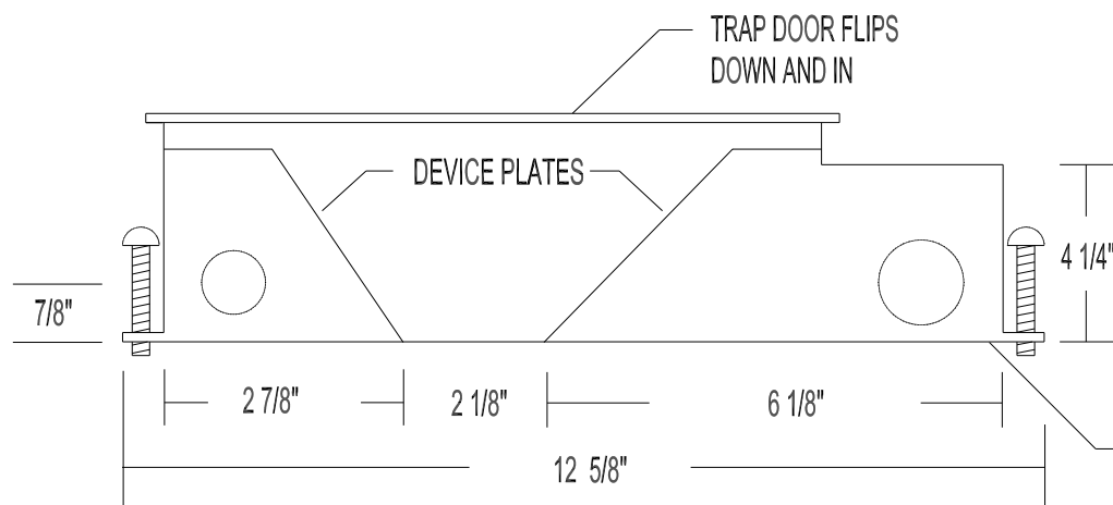
END VIEW
