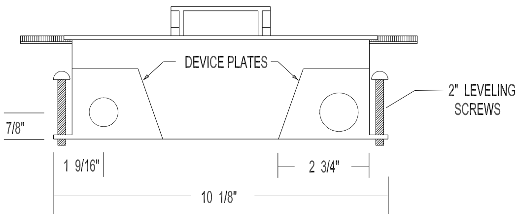
END VIEW
