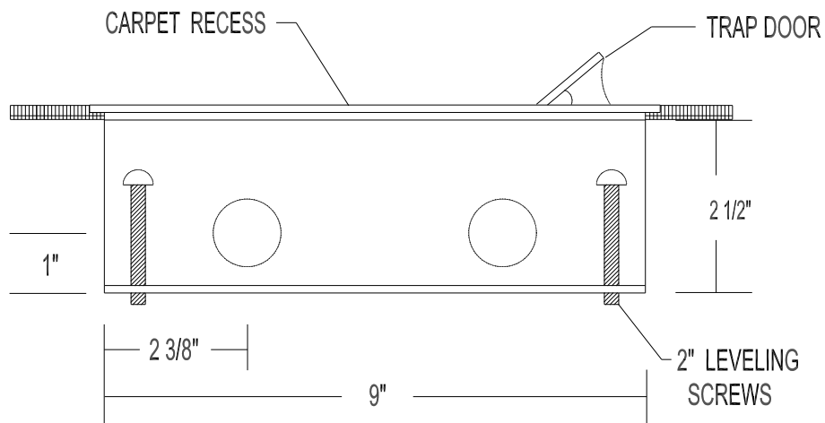
SIDE VIEW
