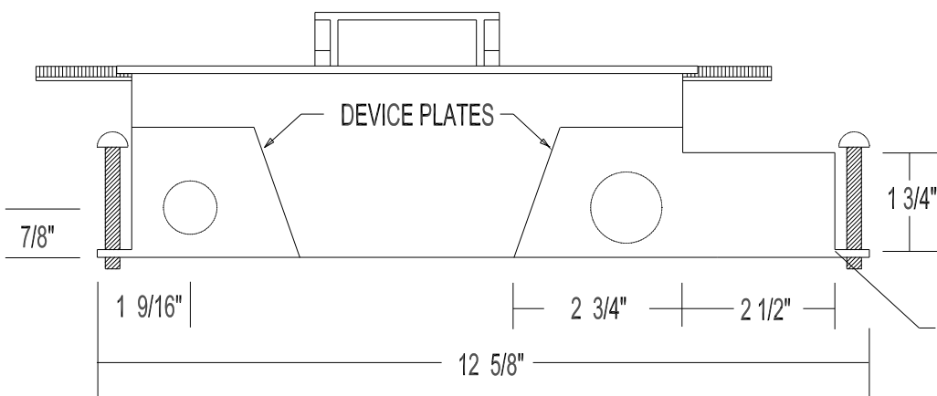
END VIEW
